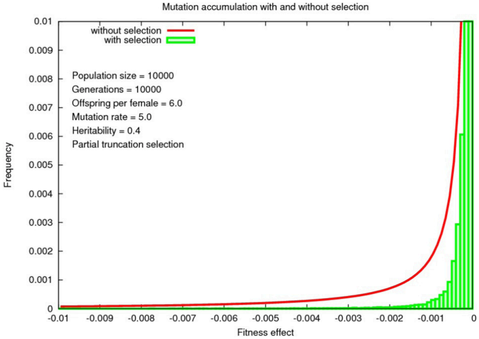
Fig. 5. Mutation distribution as a function of fitness effect, shown on a linear scale. The case is the same as shown in Fig. 4. The curved line is the theoretical distribution with no selection. The histogram is the actual mutation distribution given intense selection. Note that only a small portion of the vertical and horizontal scales is displayed.
